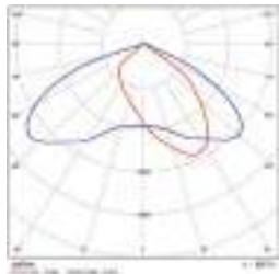
Asimétrica LED Outdoor Orion 50W-100W
